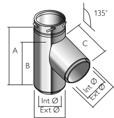
135° Tee
